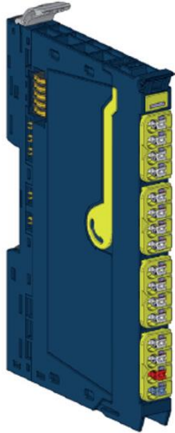
Figure 13: Safe Power-feed Module EP-1922
