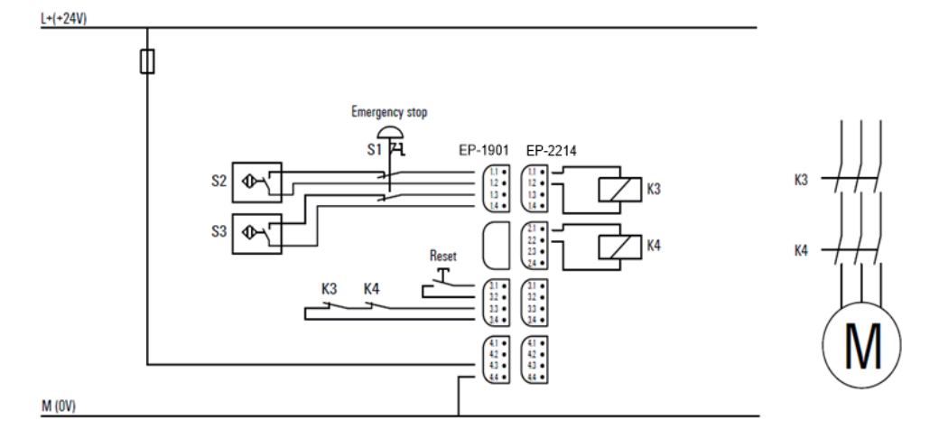
Figure 27: Example Application for Dual-channel Safety Door Monitoring with Proximity Detectors, Automatic Reset and Emergency Stop
