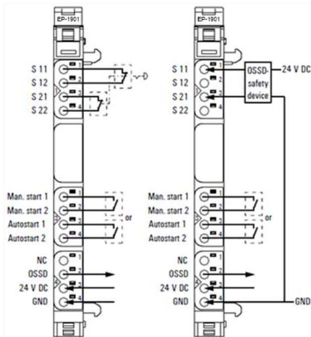
Figure 7: Connection Diagram
