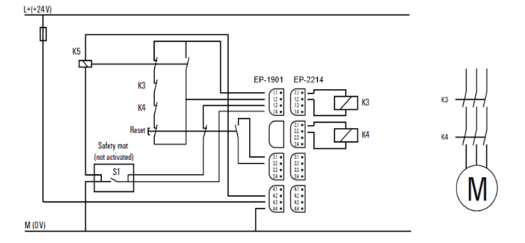
Figure 22: Example Application for Safety Mat
