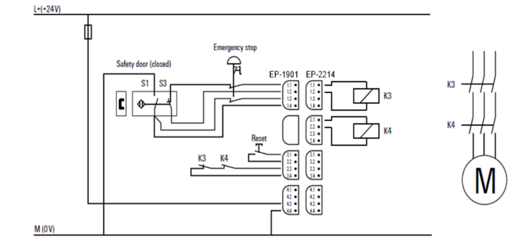
Figure 24: Example Application for Dual-channel Safety Door Monitoring with Magnetic Switch, Automatic Reset and Emergency Stop
