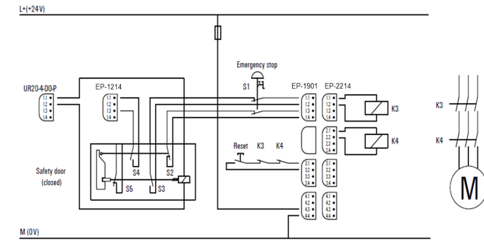
Figure 26: Example Application for Dual-channel Safety Door Monitoring, Magnetically Operated Interlock with Manual Reset, Stop and Emergency Stop
