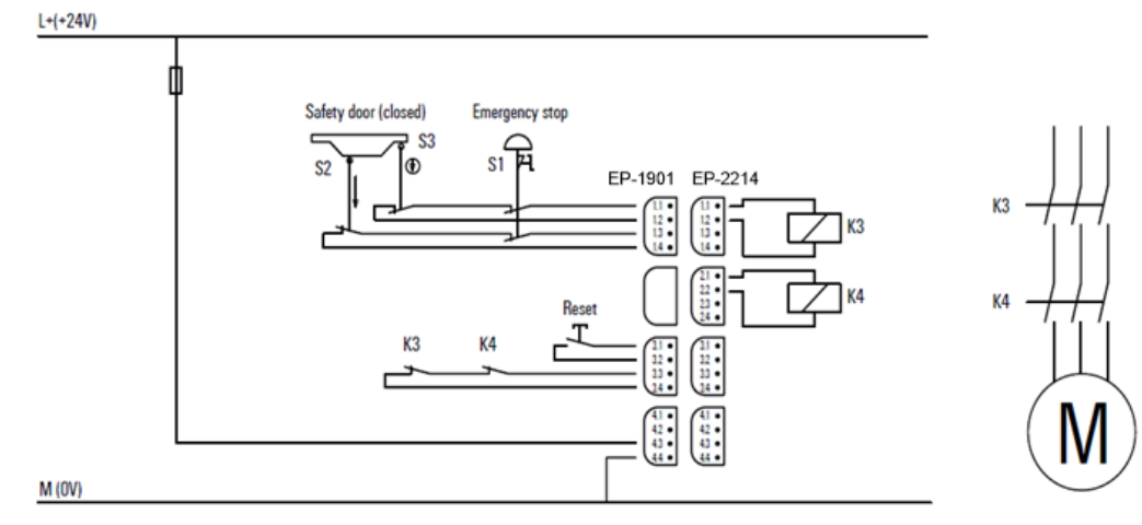
Figure 21: Example Application for Dual-channel Safety Door Monitoring with Automatic Reset & Emergency Stop
